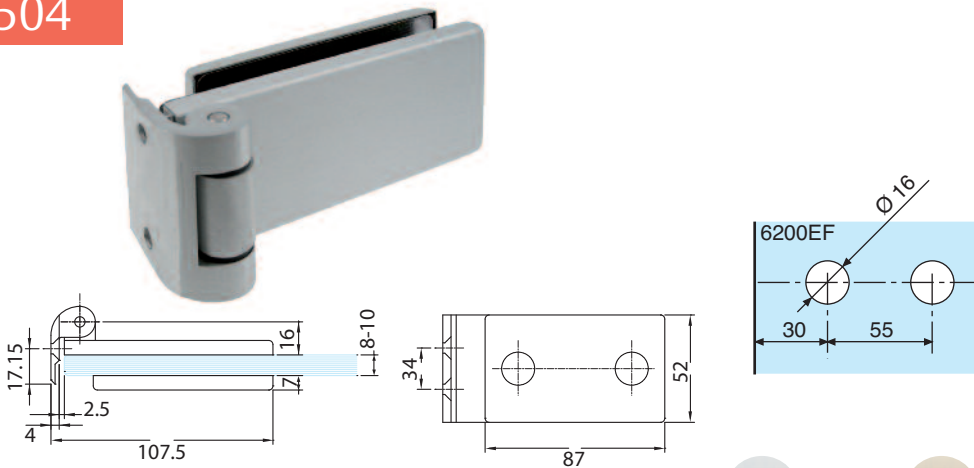
Aluminium anodisé Argent Brossé / Brushed anodised alu silver Aluminium anodisé Aninox / Brushed anodised alu.
