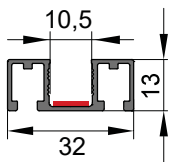
⑤ Guida porta DIV-012 Door guide DIV-012 Bodenführung DIV-012
