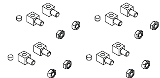
④ Kit assemblaggio P-F37 Assembly kit P-F37 Montage-Kit P-F37
