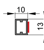
③ Traversino DIV-204 Cross profile DIV-204 Querprofil DIV-204
