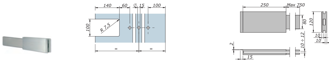
Contro per Art. 270 con fasce Lock keeper for Art. 270 with cable cover
