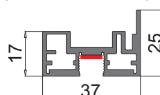
④ DIV-104 MONTANTE VERTICALE (porta doppia lato contropiastra) VERTICAL PROFILE (double hinged door, strike plate side) VERTICAL PROFILE (2 FLG - Schließblechseite)
