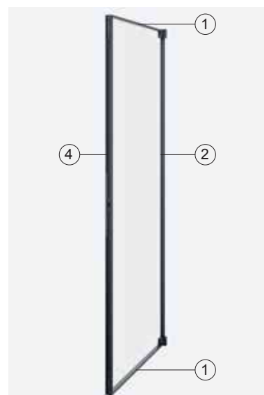
④ DIV-104 MONTANTE VERTICALE (porta doppia lato contropiastra) VERTICAL PROFILE (double hinged door, strike plate side) VERTICAL PROFILE (2 FLG - Schließblechseite)
